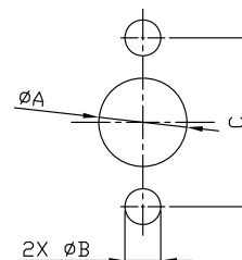
Mounting Dimension
